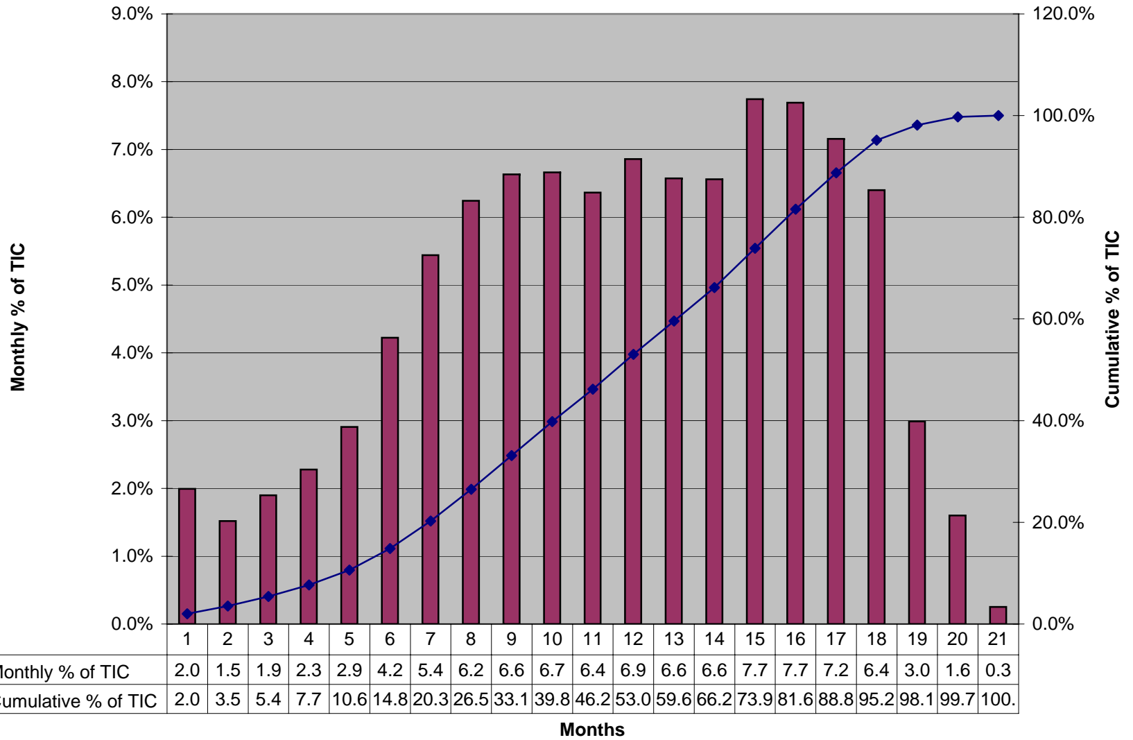
Typical Spend Out Curve as a % of Total Installed Cost ( TIC )
